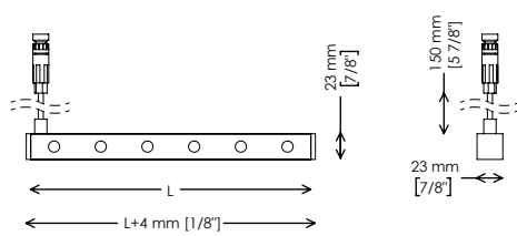
LEFT-SIDE FEED
