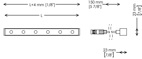
BOTTOM FEED
