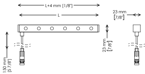
RIGHT-SIDE FEED
